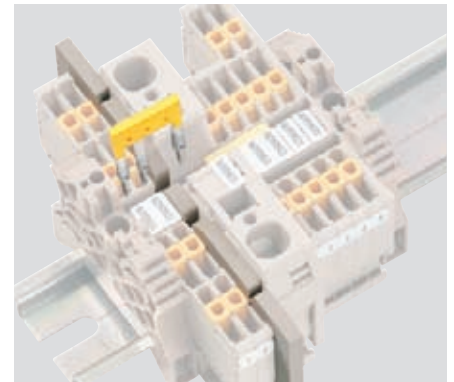
Power supply with the IEPL feed plate
