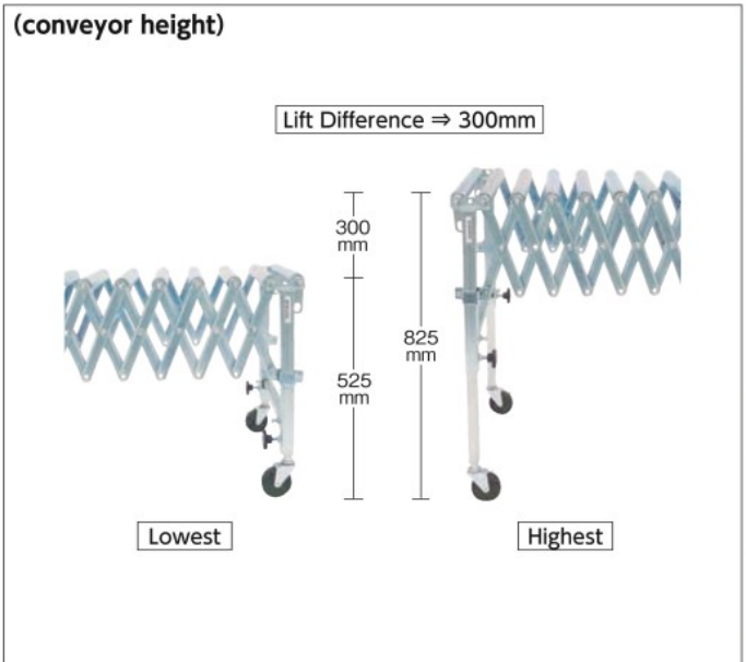
It is easy to match the height with the pitch mark on the leg extendable part.
