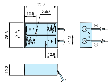
N cell×2
