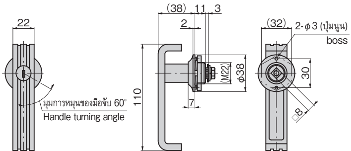
กุญแจ No.0200 Key
