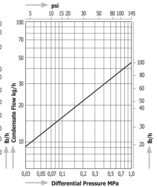
Capacity Chart SL3
