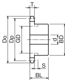
B-Type Ground Specification
