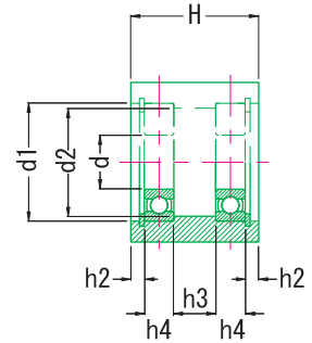
MCF-55 Type
