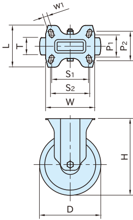
CAF8-PBL CAF8-PBL-SUS (Fixed Bracket)
