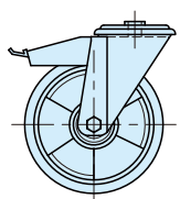
CAF5-FSF
